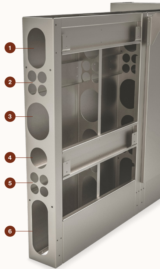
1. VENT LINE CHASE, 2. ELECTRICAL CHASE, 3. BEER CHASE, 4. SODA CHASE, 5. WATER LINE CHASE, 6. PLUMBING CHASE
